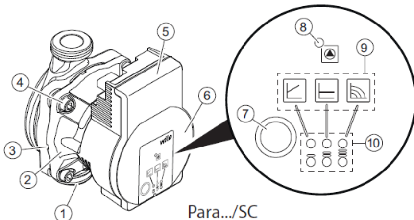
Figure 67 – Pompe Wilo
