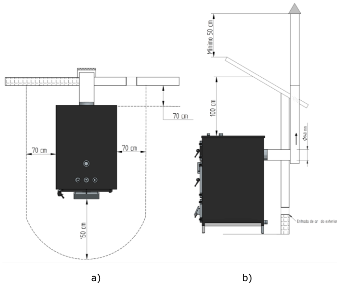
Figure 11 – Minimum distances to all surfaces: a) top view of the installation of equipment; b) side view of the installation device
