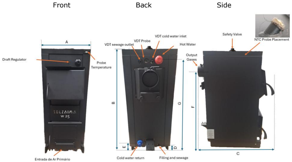
Figure 2 - Hydraulic connections
